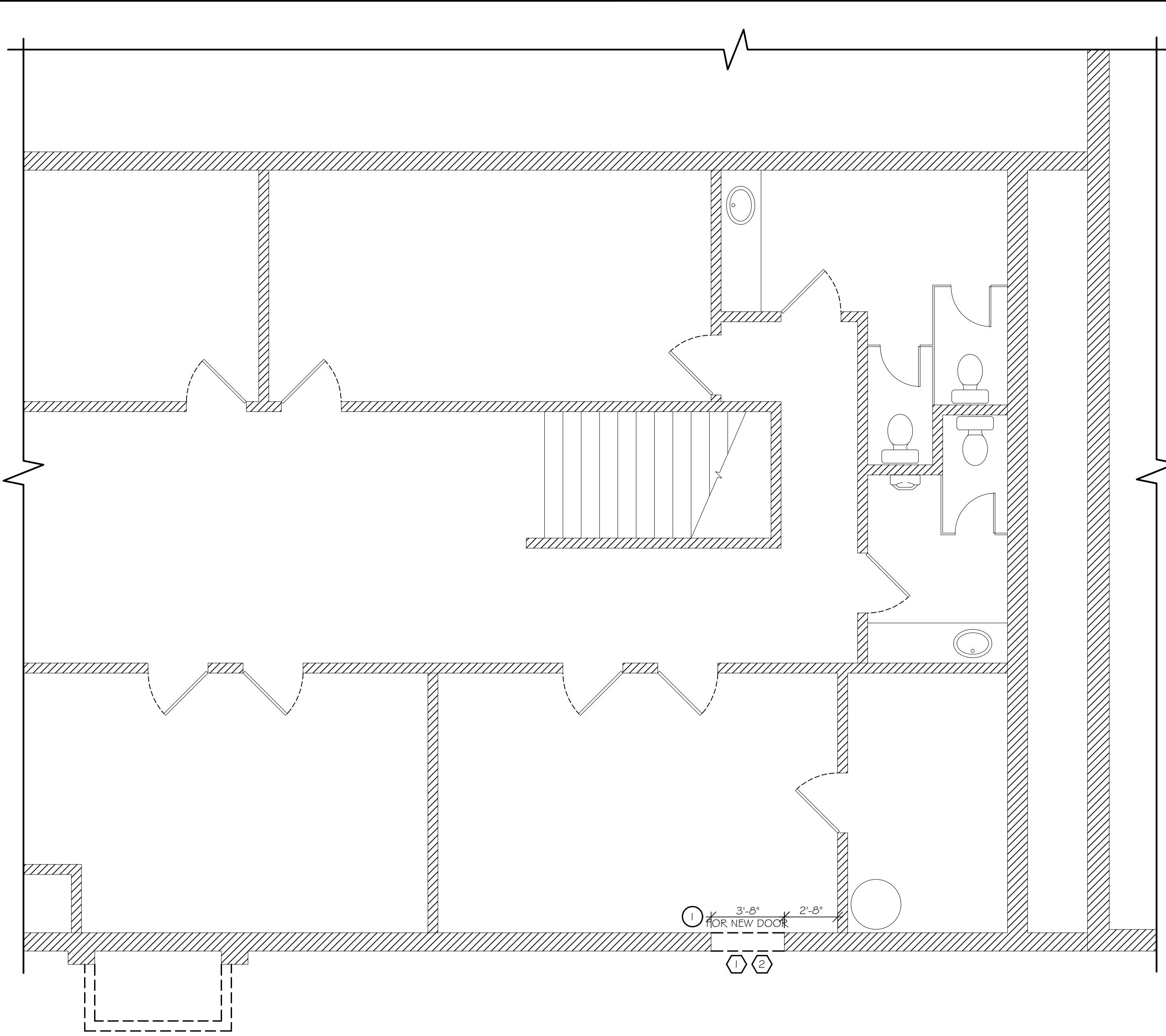
3 BASEMENT PLAN SCALE 1/4" = 1'-0" DEMOLITION
