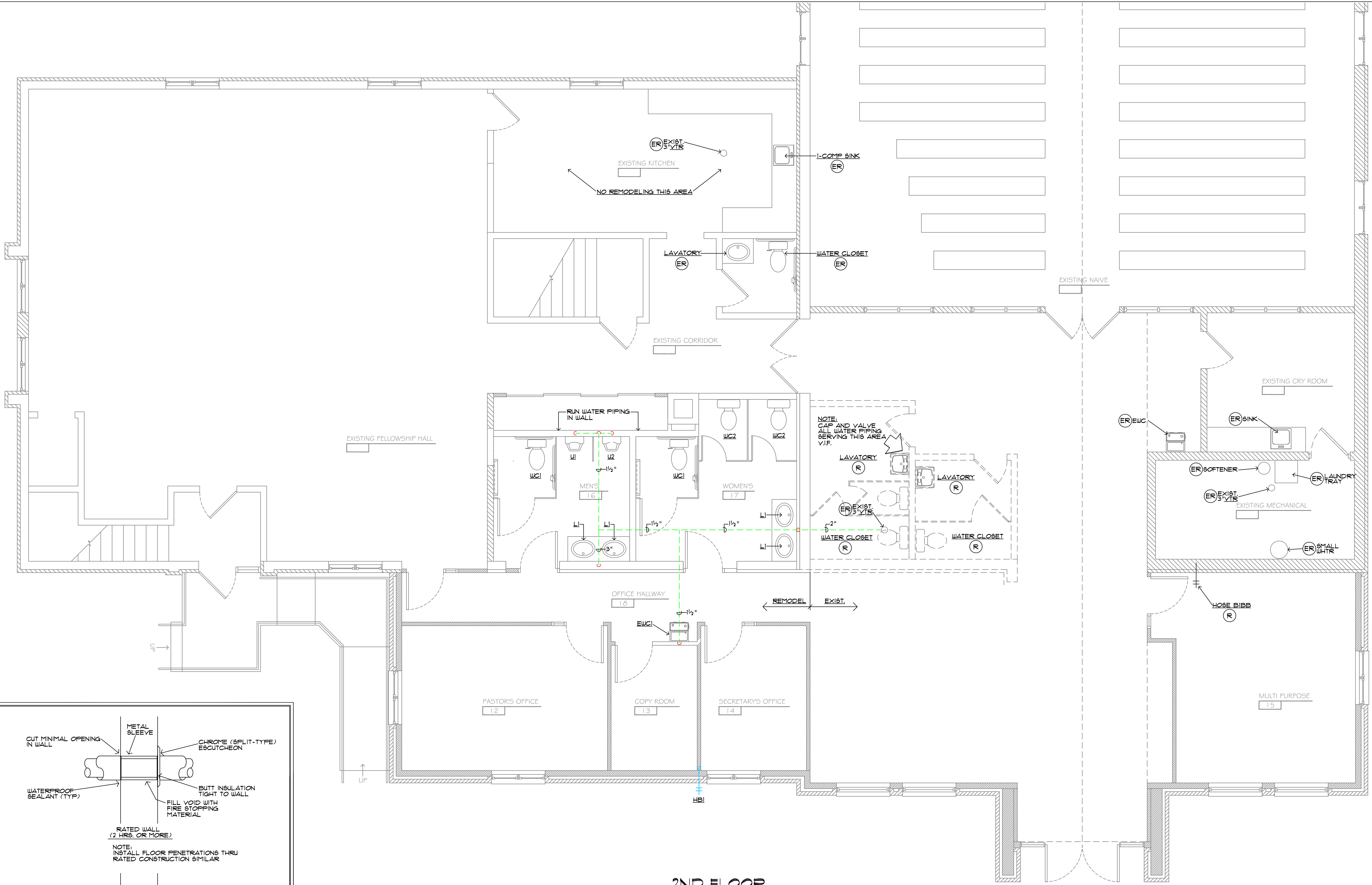
2ND FLOOR PLUMBING PLAN SCALE: 1/4" = 1' - 0" NORTH
